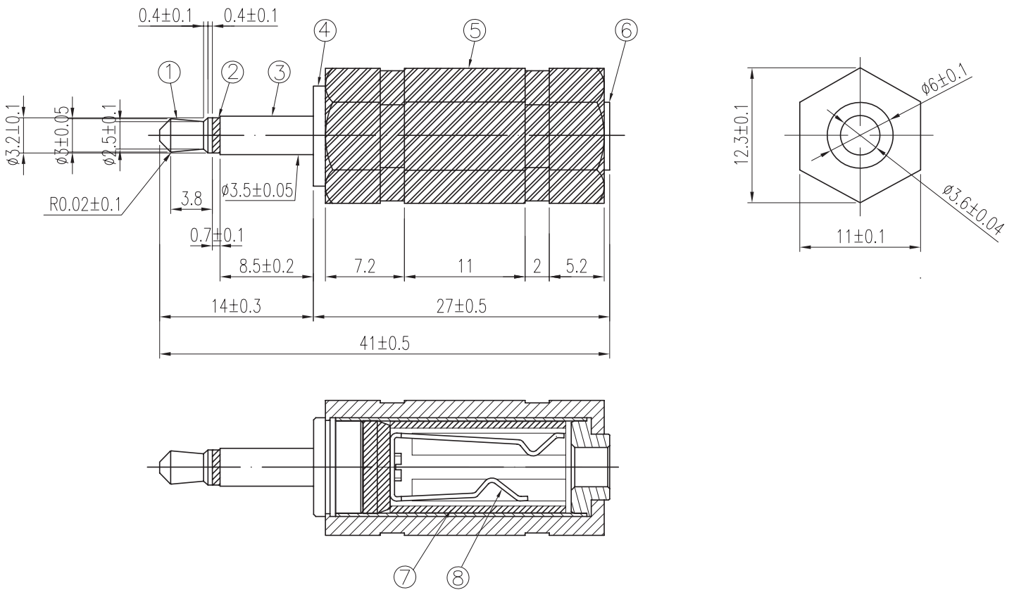
Ø3.5 Mono Plug
