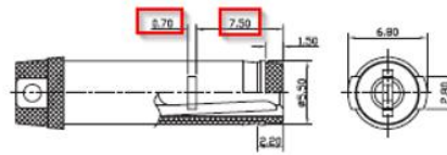
MATING PLUG Jack Insertion Depth: 9.5 mm
