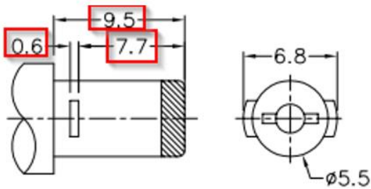
MATING PLUG Jack Insertion Depth: 9.8 mm
